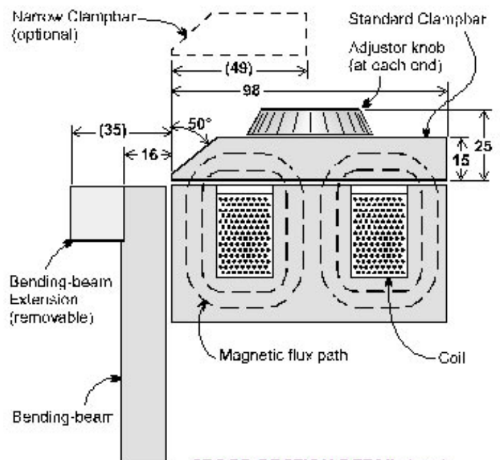
CROSS-SECTION DETAIL (mm)
